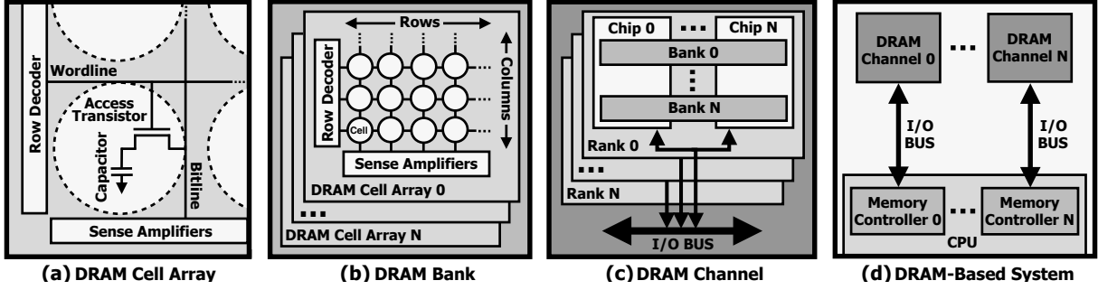
Figure 1: DRAM organization.
